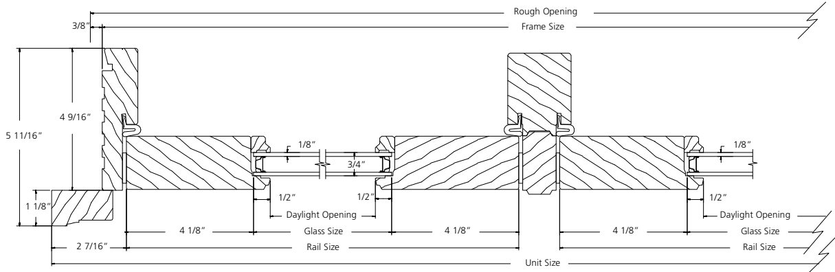
HORIZONTAL SECTION
