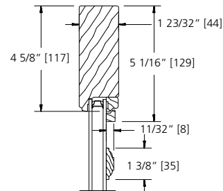
1 3/8" GRILLE BAR
