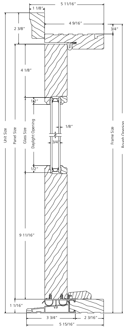
VERTICAL SECTION
