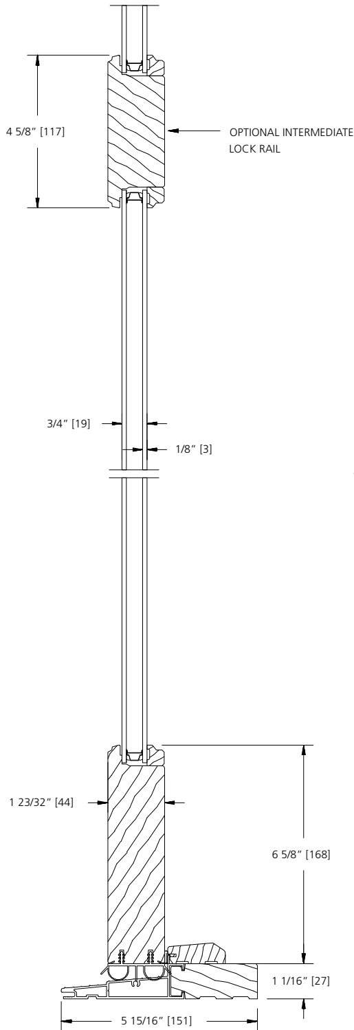
STANDARD 6 5/8\" BOTTOM RAIL STANDARD SILL (4 9/16\" / 6 9/16\" JAMB)
