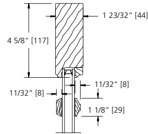
1 1/8" SDL BAR (PUTTY/BEAD)
