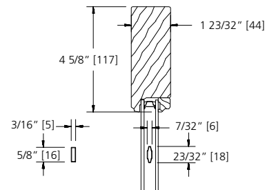
5/8" FLAT GBG
