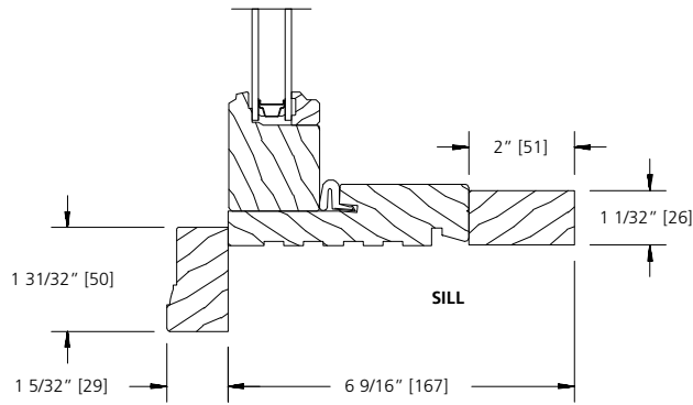
2" OPTIONAL TRANSOM SILL EXTENDER (6 9/16" JAMB)
