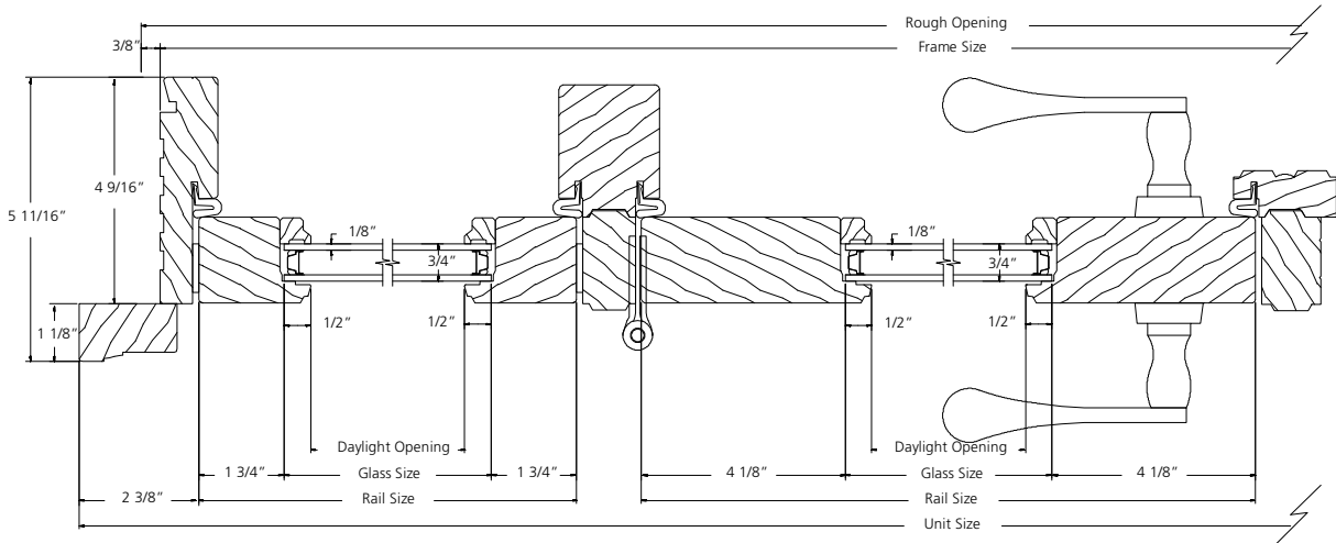
HORIZONTAL SECTION
