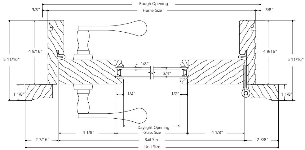
HORIZONTAL SECTION
