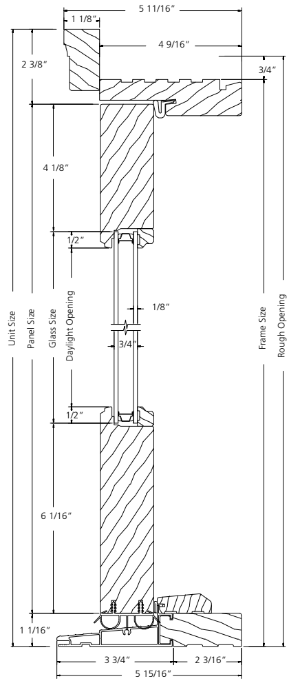
VERTICAL SECTION
