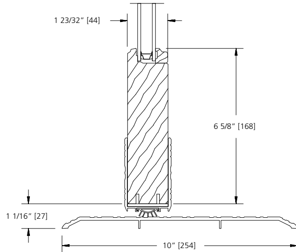
STANDARD 6 5/8\" BOTTOM RAIL HANDICAP SILL (6 9/16\" JAMB)
