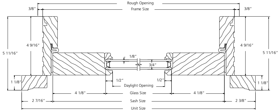
HORIZONTAL SECTION
