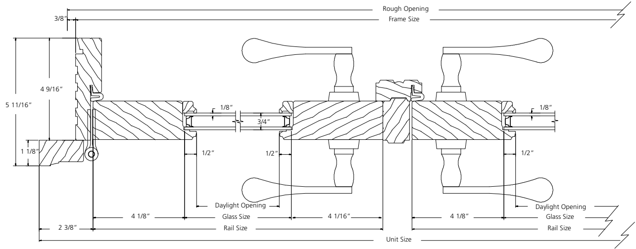
HORIZONTAL SECTION
