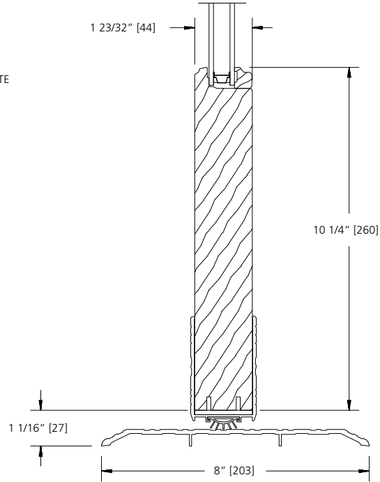
OPTIONAL 10 1/4\" BOTTOM RAIL HANDICAP SILL (4 9/16\" JAMB)
