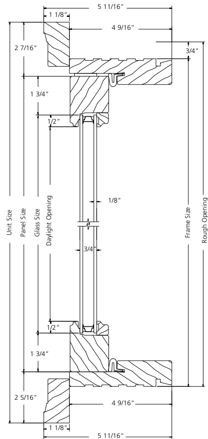
VERTICAL SECTION
