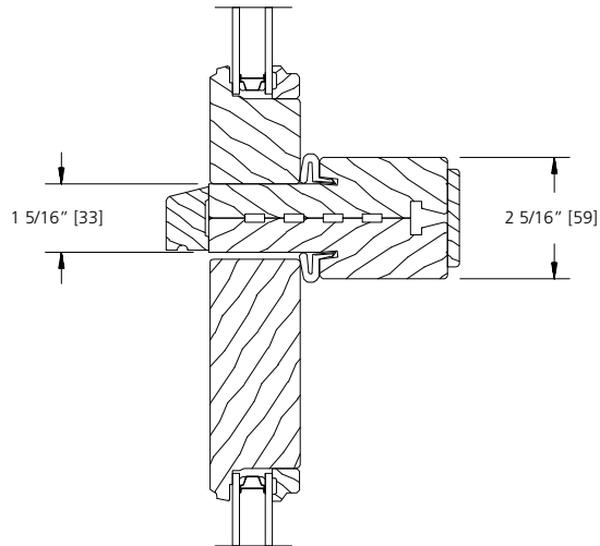
HEAD / TRANSOM SILL
