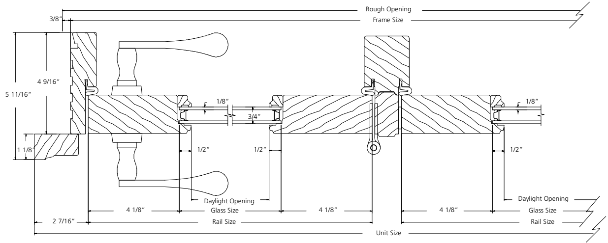
HORIZONTAL SECTION
