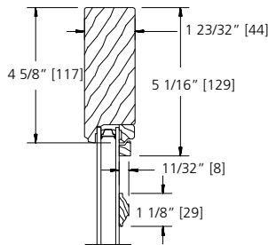
1 1/8" GRILLE BAR
