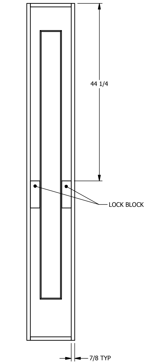
LOCK BLOCK LOCATION DOOR SKIN REMOVED
