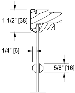
5/8" SDL (PUTTY/PUTTY)
