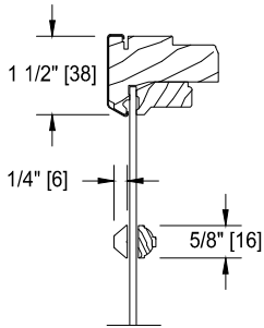
5/8" SDL (PUTTY/BEAD)
