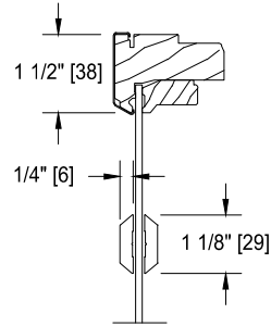
1 1/8" SDL (PUTTY/PUTTY)
