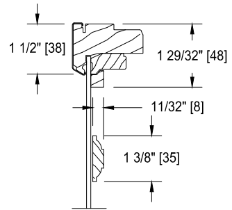
1 3/8" GRILLE BAR
