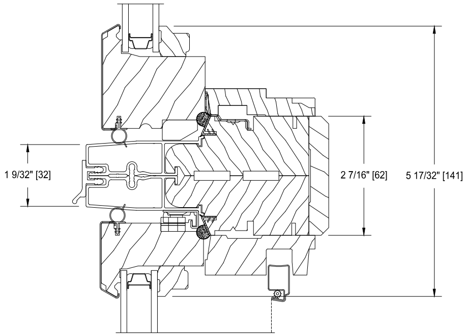
HEAD/SILL
