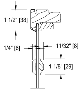
1 1/8" SDL (PUTTY/BEAD)
