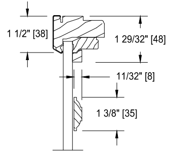
1 3/8" GRILLE BAR
