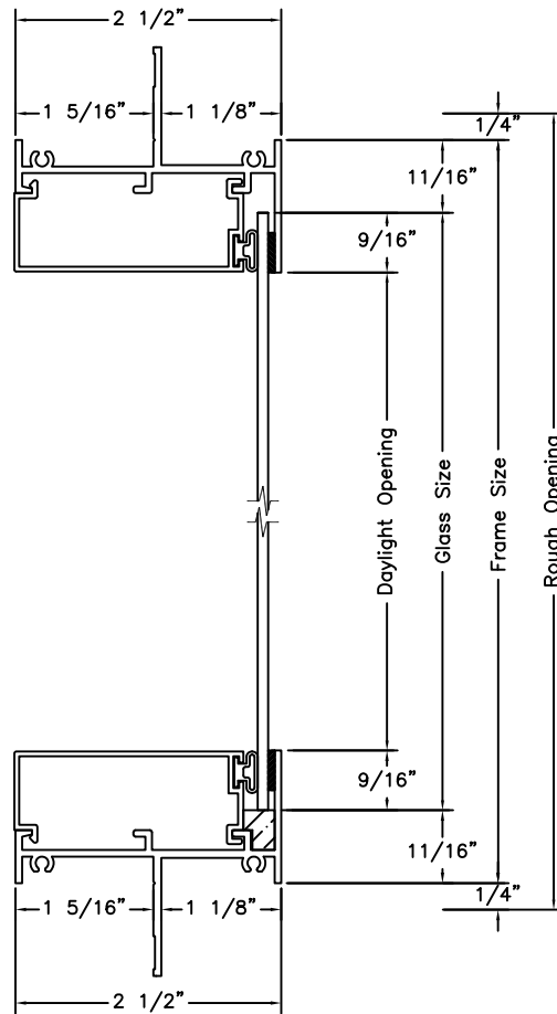
Vertical Section
