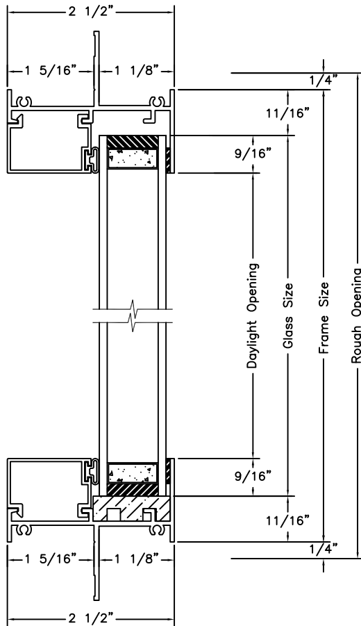
Vertical Section
