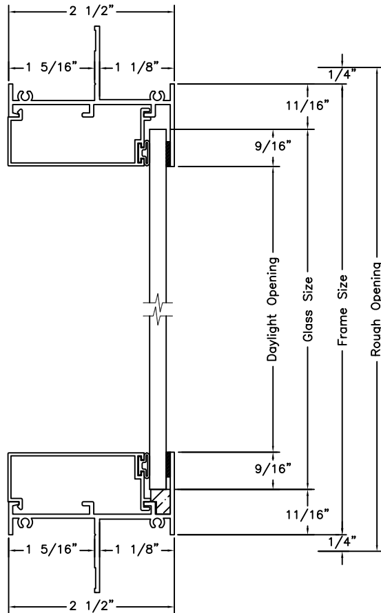
Vertical Section
