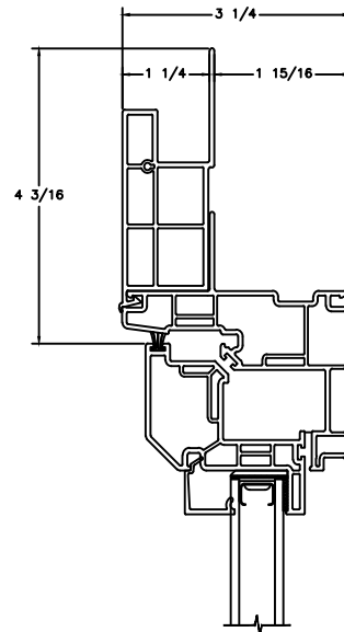
FLAT CASING
