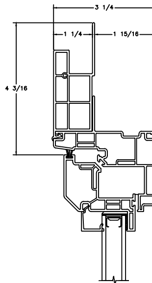
FLAT CASING
