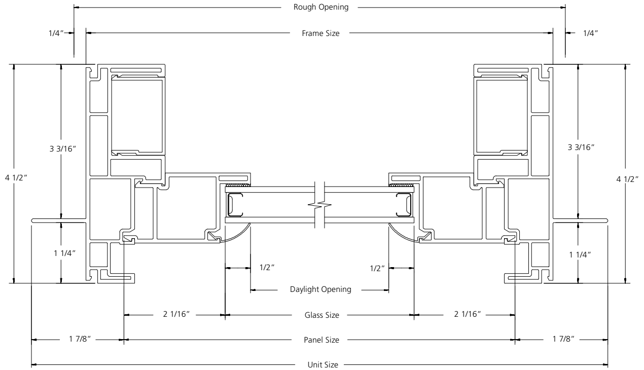
HORIZONTAL SECTION
