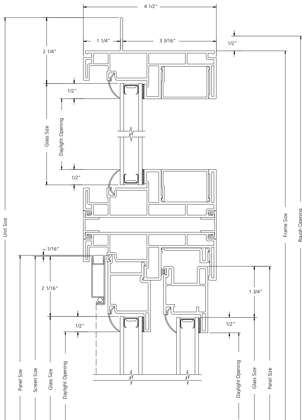
VERTICAL SECTION
