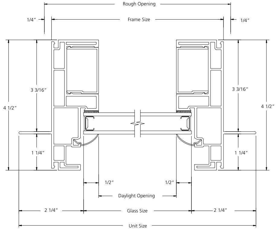
HORIZONTAL SECTION
