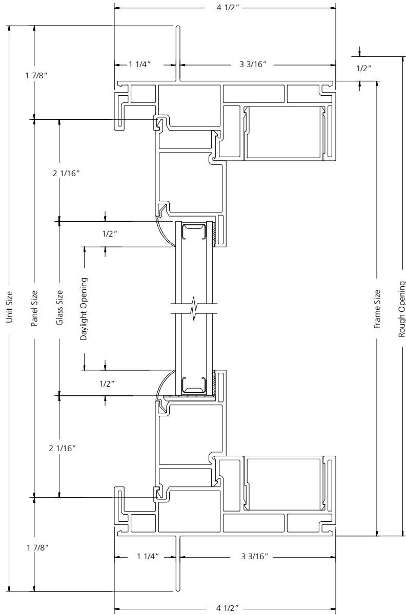
VERTICAL SECTION
