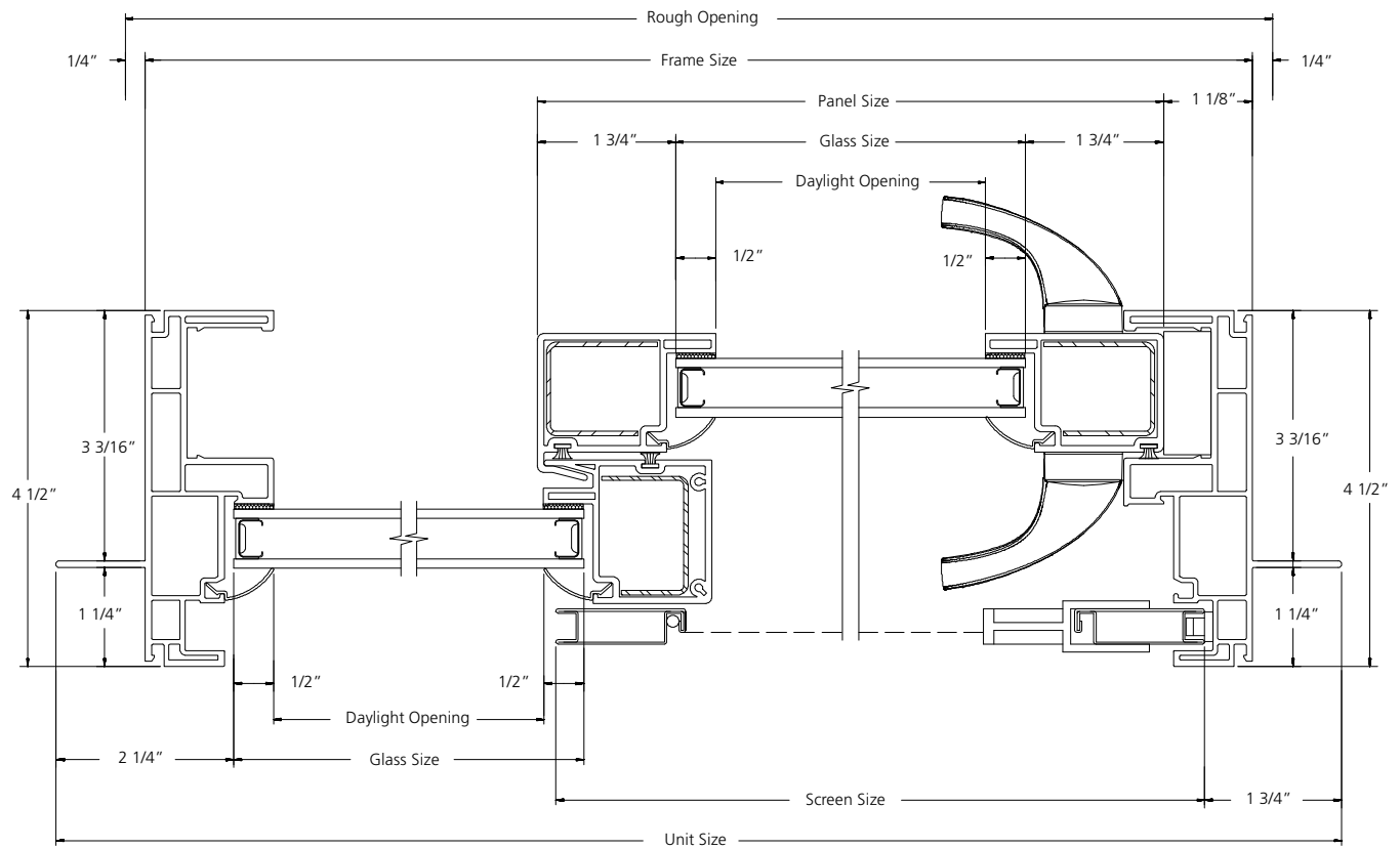
HORIZONTAL SECTION
