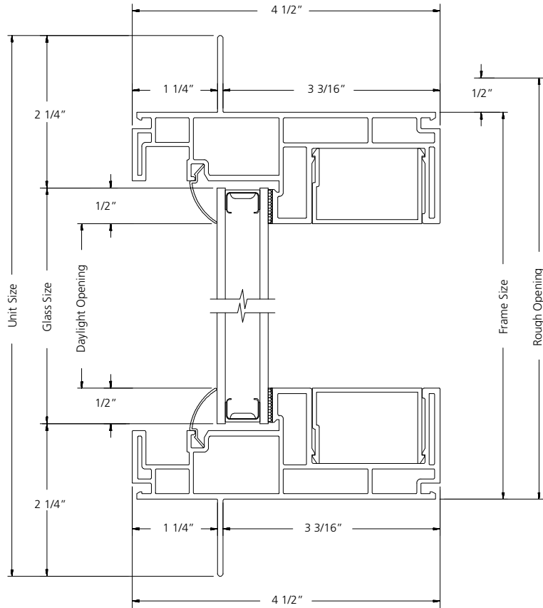
VERTICAL SECTION
