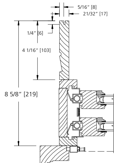
8 5/8" WALL 4/4 JAMB THICKNESS (STANDARD) KERFED EXTENSION SHOWN
