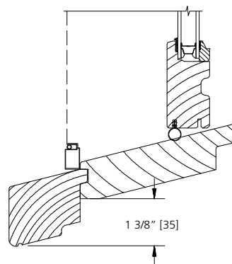
2" NOSING
