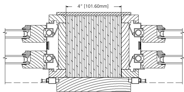
4" WOOD SPREAD MULLION
