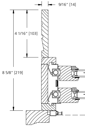
8 5/8" WALL
