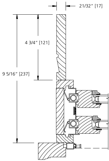
9 5/16" WALL
