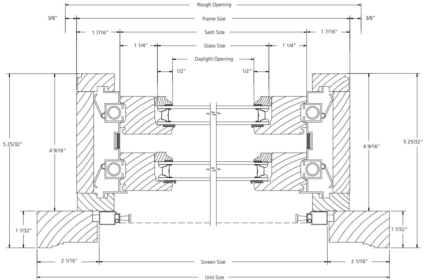
HORIZONTAL SECTION
