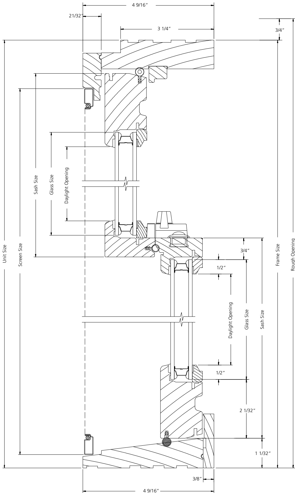
VERTICAL SECTION
