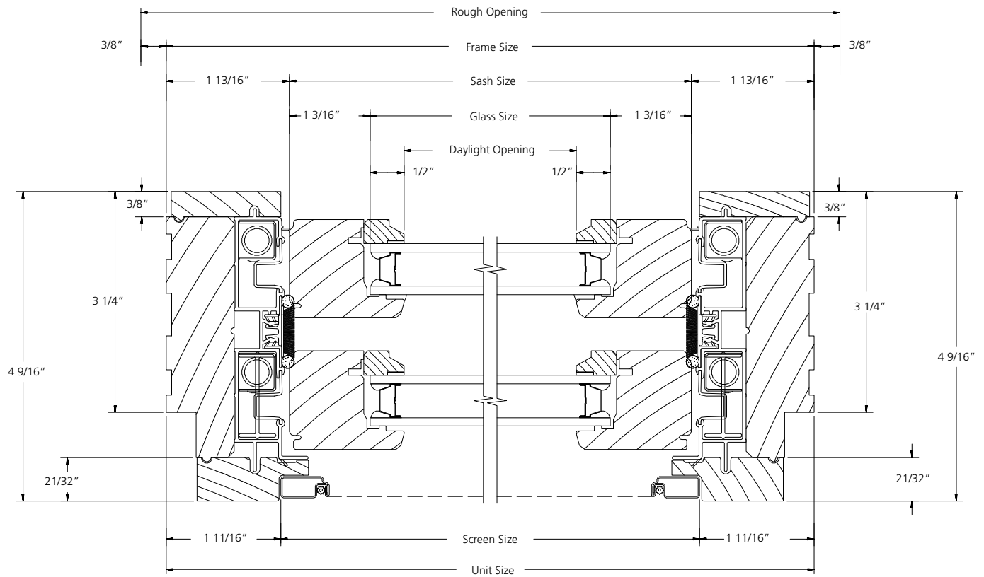
HORIZONTAL SECTION
