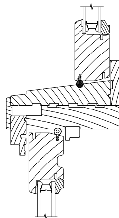
FIXED OVER POCKET DOUBLE-HUNG
