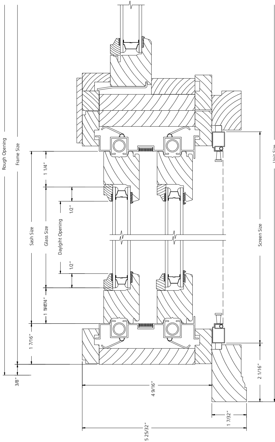
HORIZONTAL SECTION
