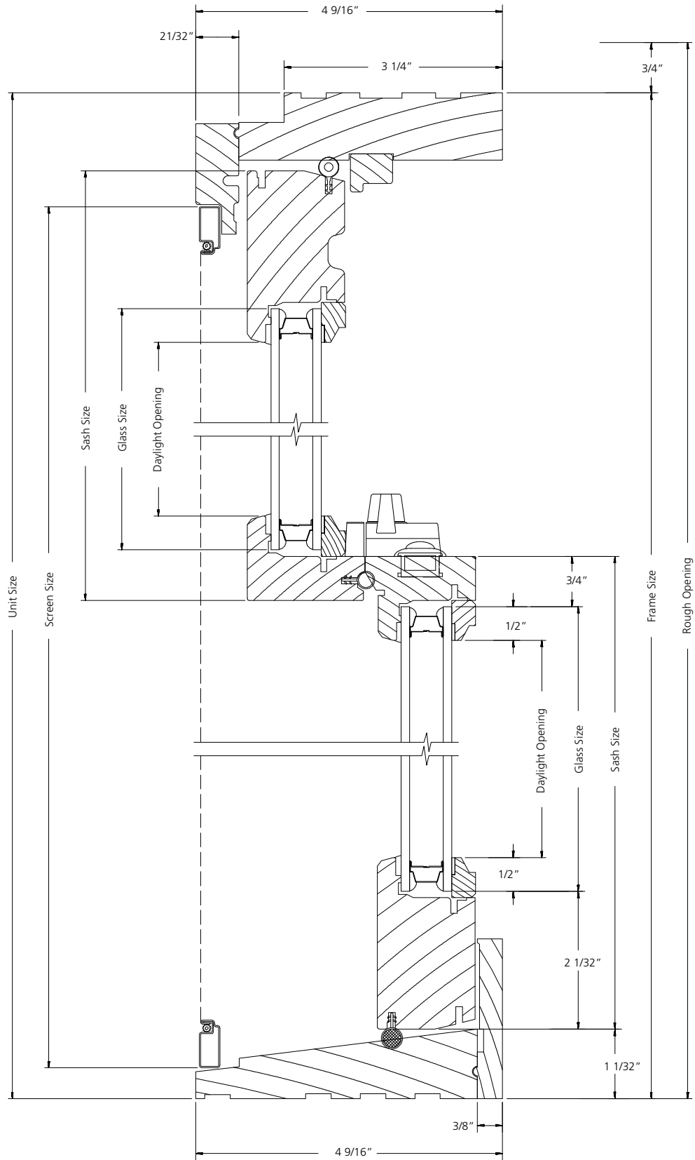
VERTICAL SECTION
