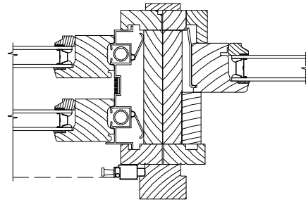
DOUBLE HUNG WITH DOUBLE HUNG PICTURE
