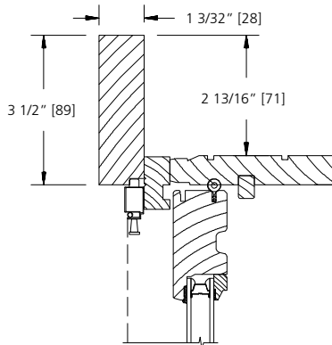
3 1/2" FLAT CASING
