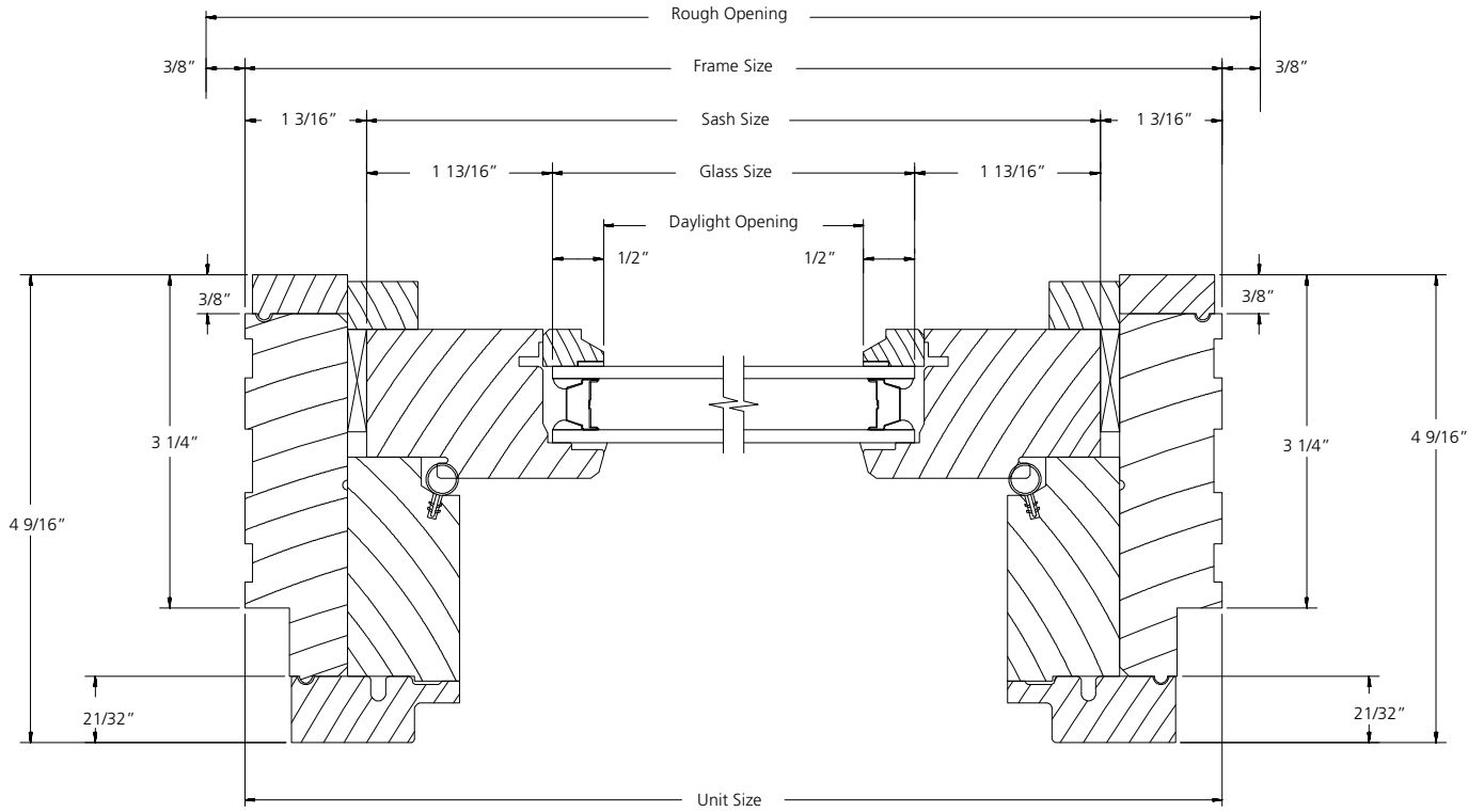
HORIZONTAL SECTION
