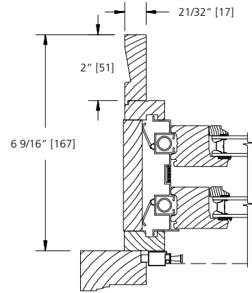
6 9/16" WALL 4/4 JAMB THICKNESS (STANDARD)
