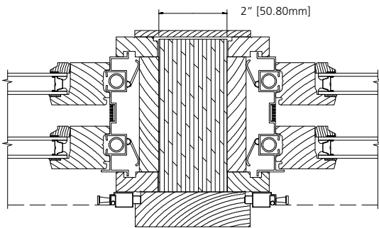
2" WOOD SPREAD MULLION
