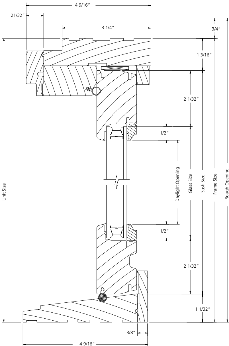
VERTICAL SECTION
