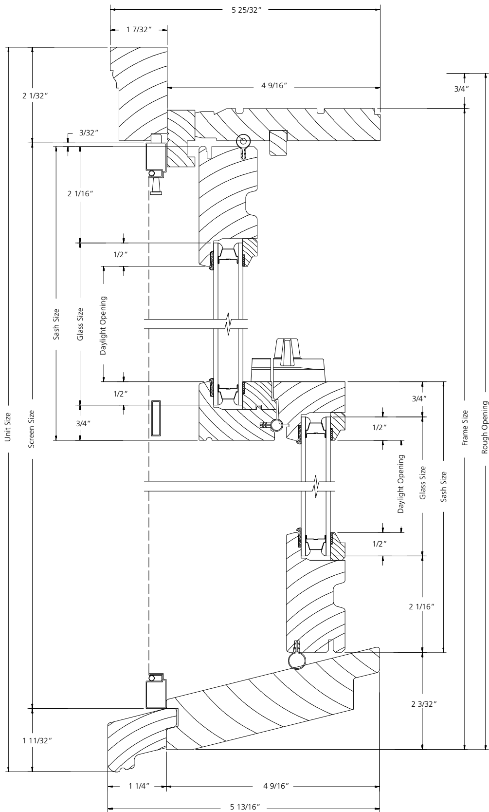
VERTICAL SECTION
