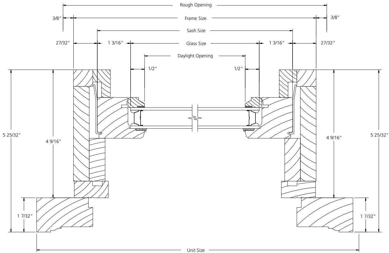
HORIZONTAL SECTION
