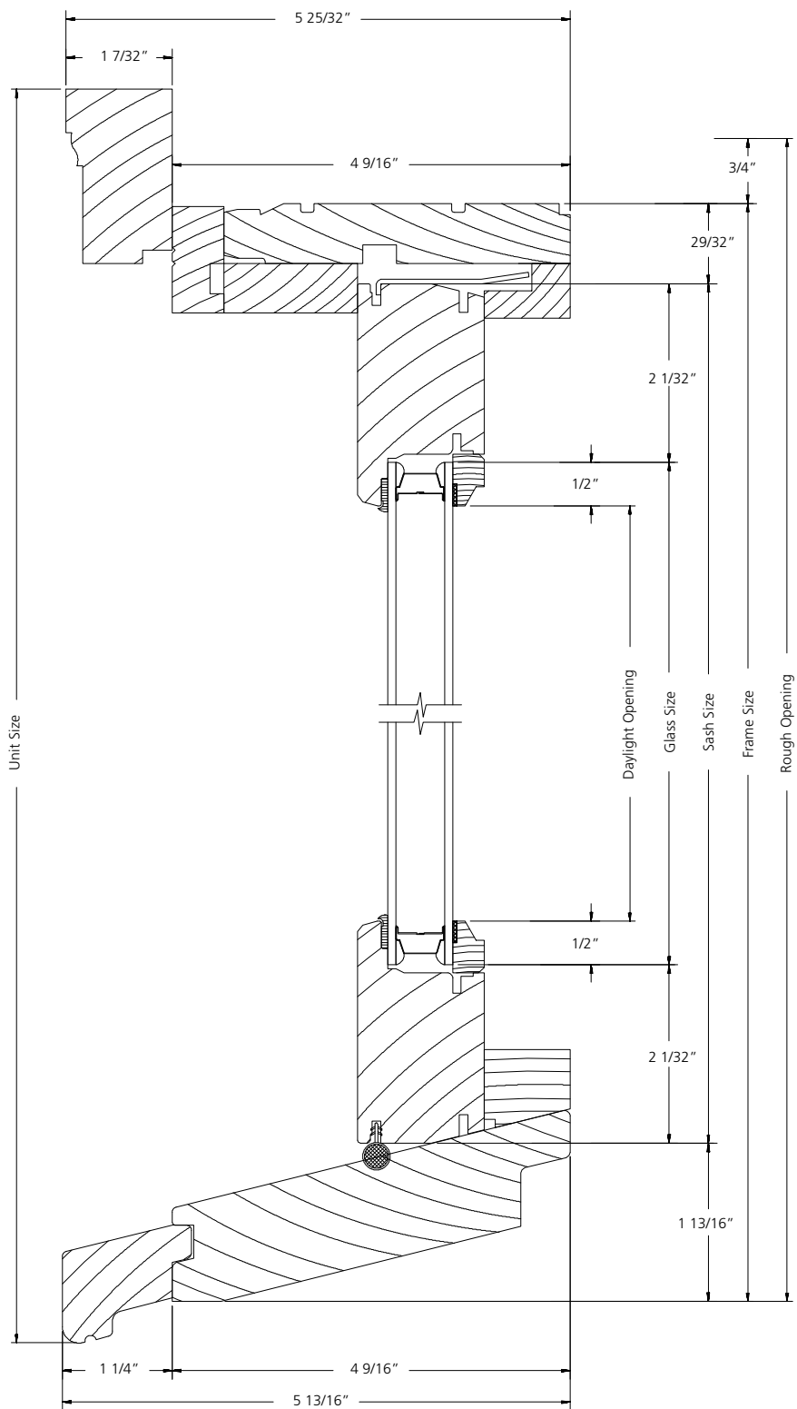
VERTICAL SECTION
