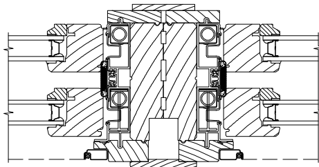
TWIN OPERATING POCKET DOUBLE-HUNG
