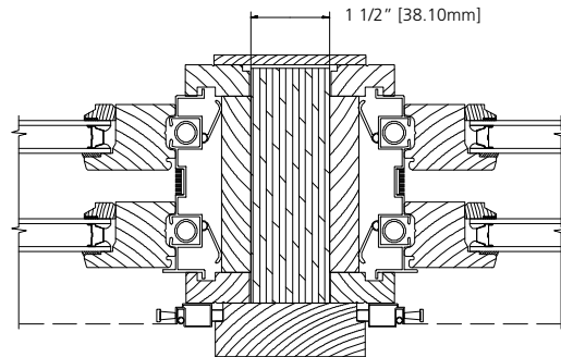
1 1/2" WOOD SPREAD MULLION
