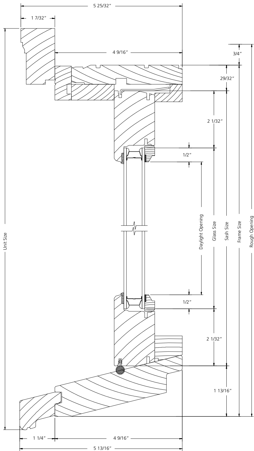
VERTICAL SECTION
