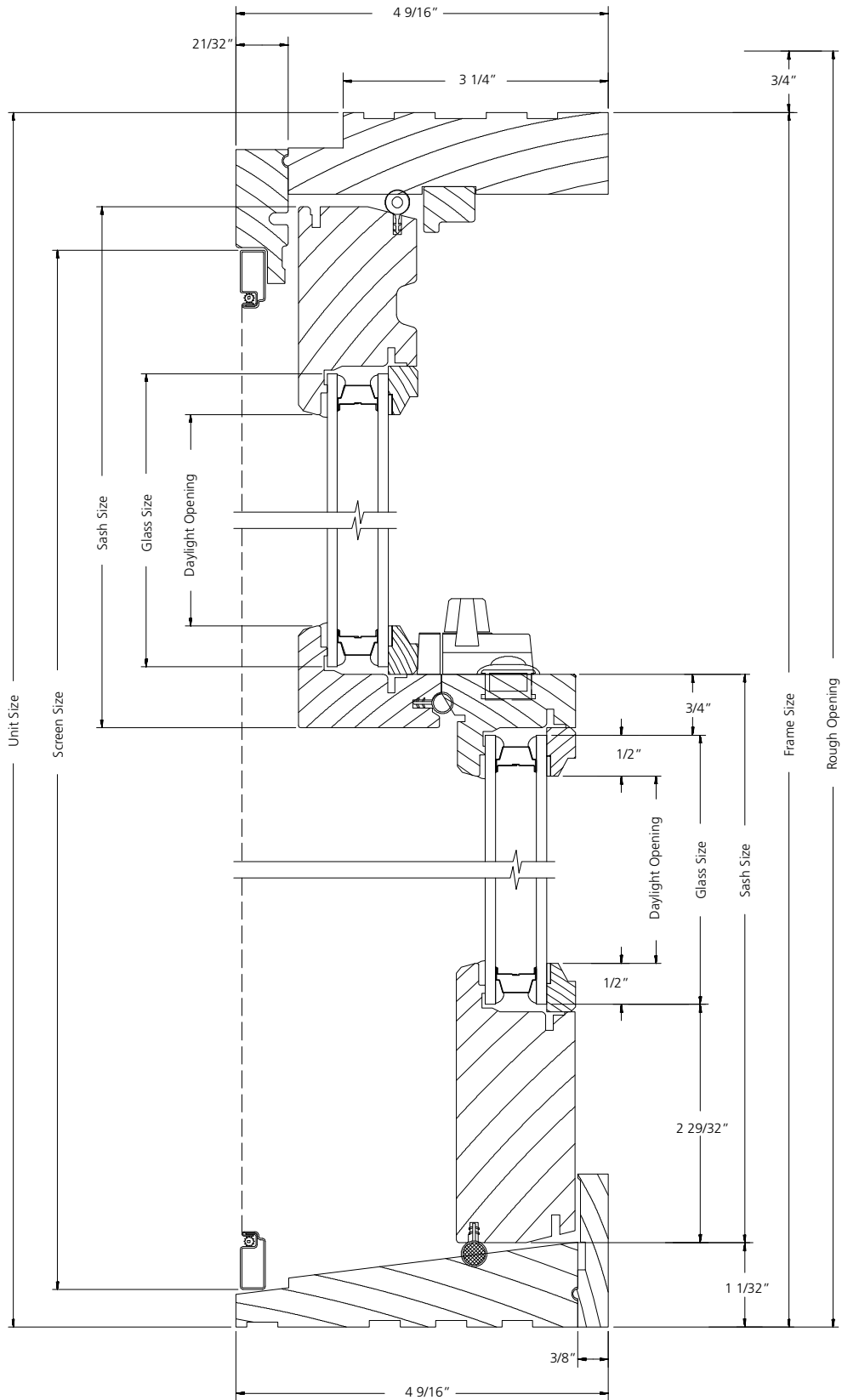
VERTICAL SECTION
