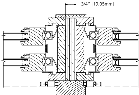
3/4" WOOD SPREAD MULLION
