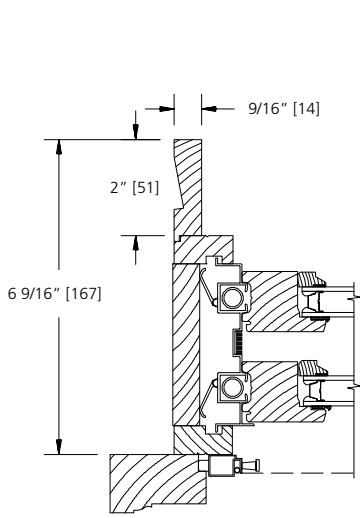
6 9/16" WALL 9/16" JAMB THICKNESS (OPTION)
